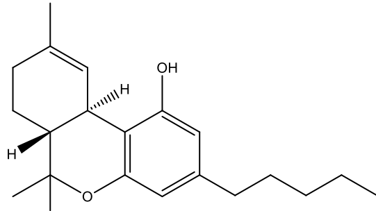
\Delta^9 -Tetrahydrokannabinol
