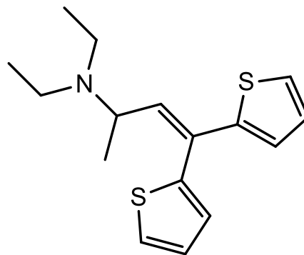
Dietylotiambuten
