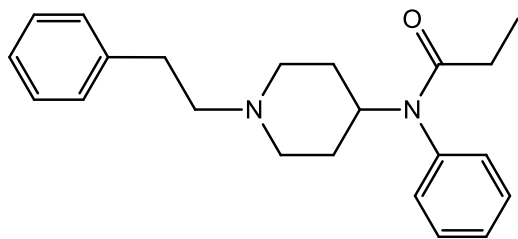
Fentanyl
