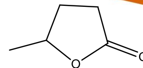
GVL
