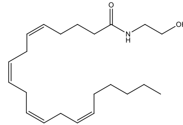
Anandamid endokannabinoid
