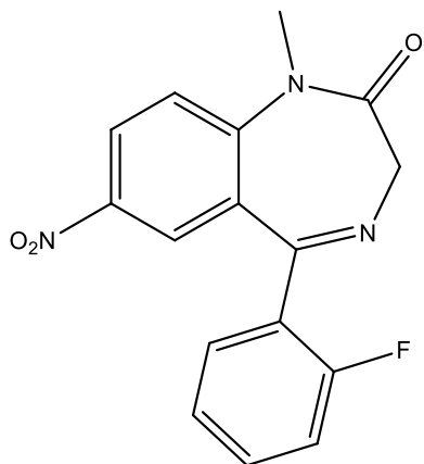
Flunitrazepam
