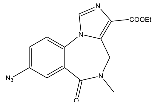
GVL
