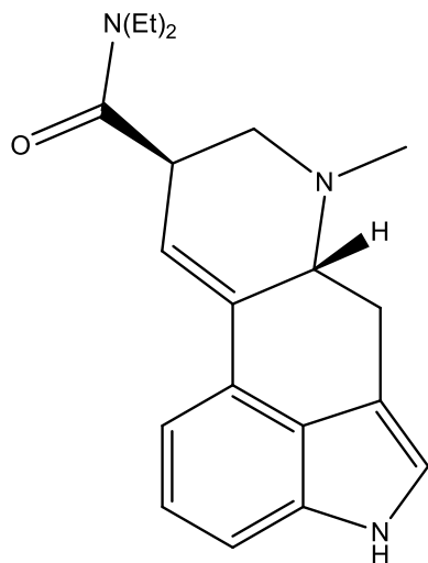
LSD
