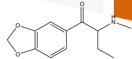
Pentylon, bk-MBDP
