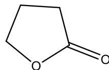
GBL
