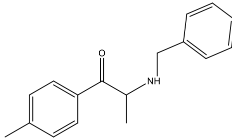
Benzedron, 4-MBC
